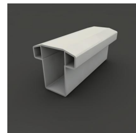
3.5"x3.5" T-Rail T: 0.11"
